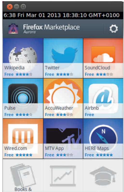
Slika 3: Firefox Marketplace
