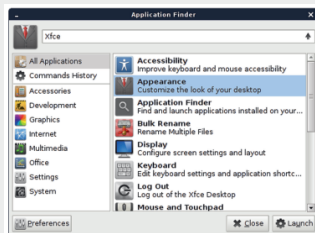
Slika 2: Application finder
