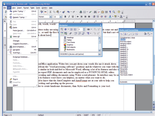
Slika 16: OpenOffice
